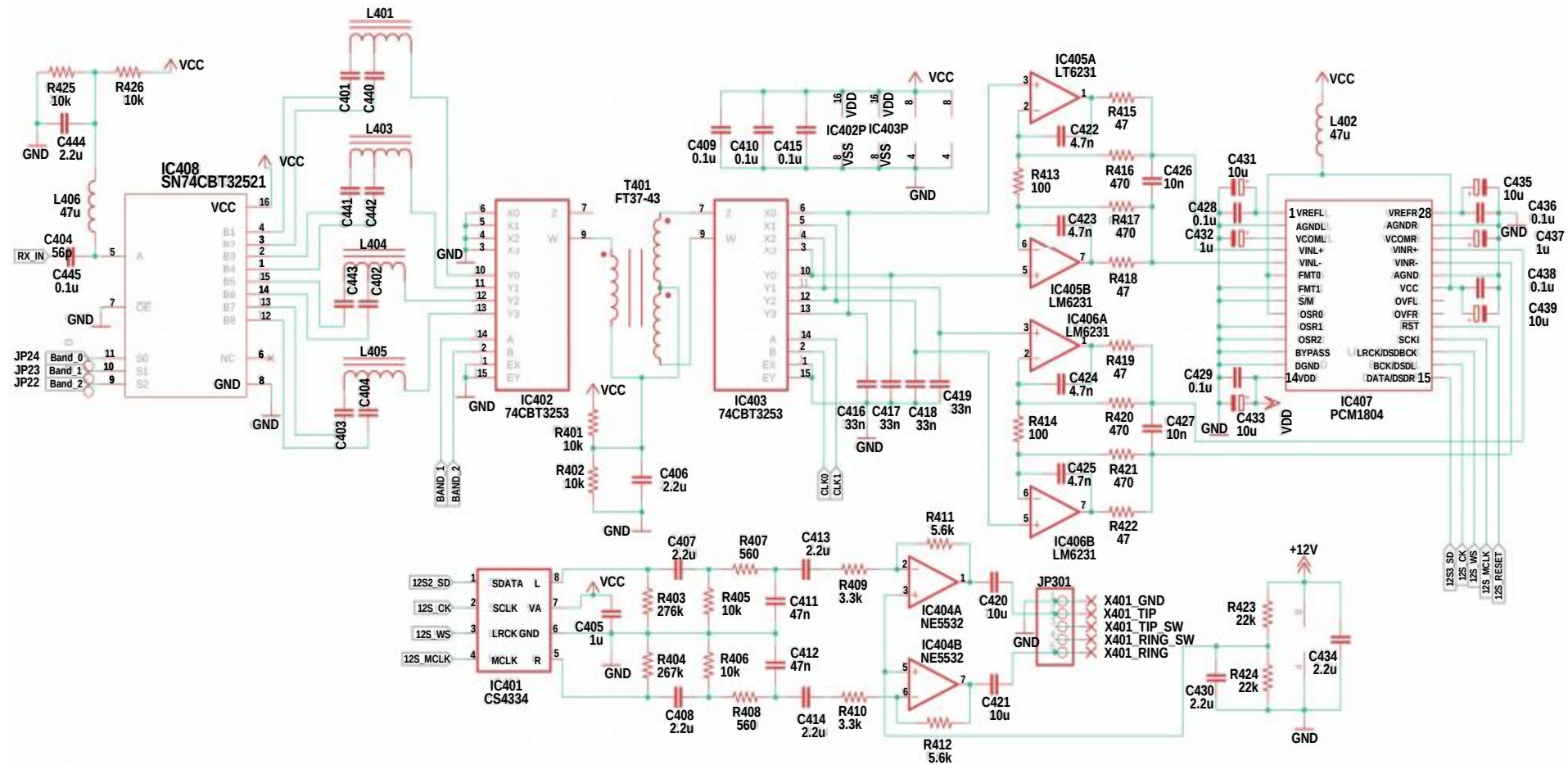
QMX+ Rev 1 Searchable Schematic 1b. Compiled by G4GIR 16 th February 2025
