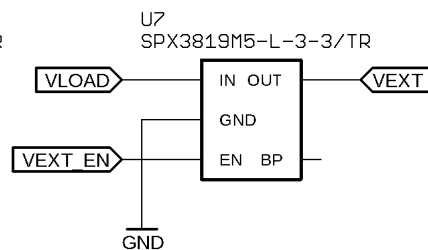
3V3 Regulator VEXT
