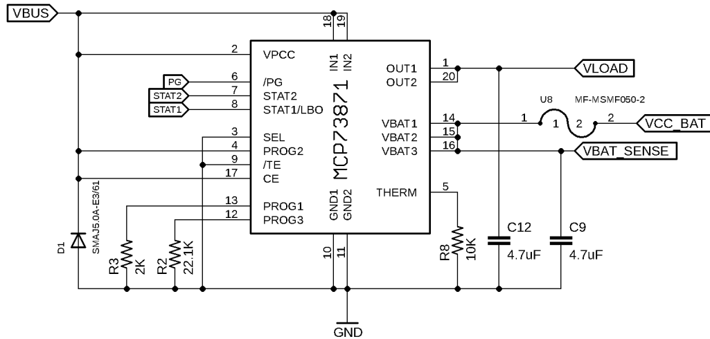
Powerpath
