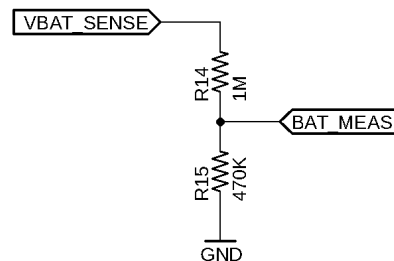
BAT MEAS ADC
