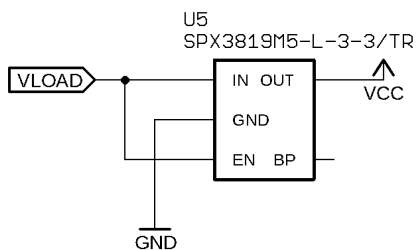
3V3 Regulator
