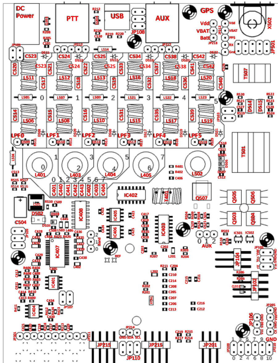
QMX+ Main board layout, top side:
