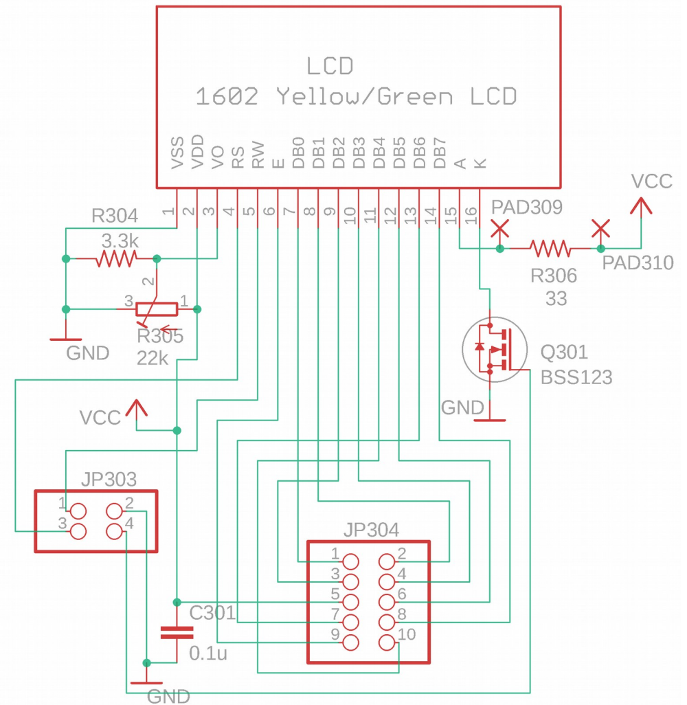
LCD board
