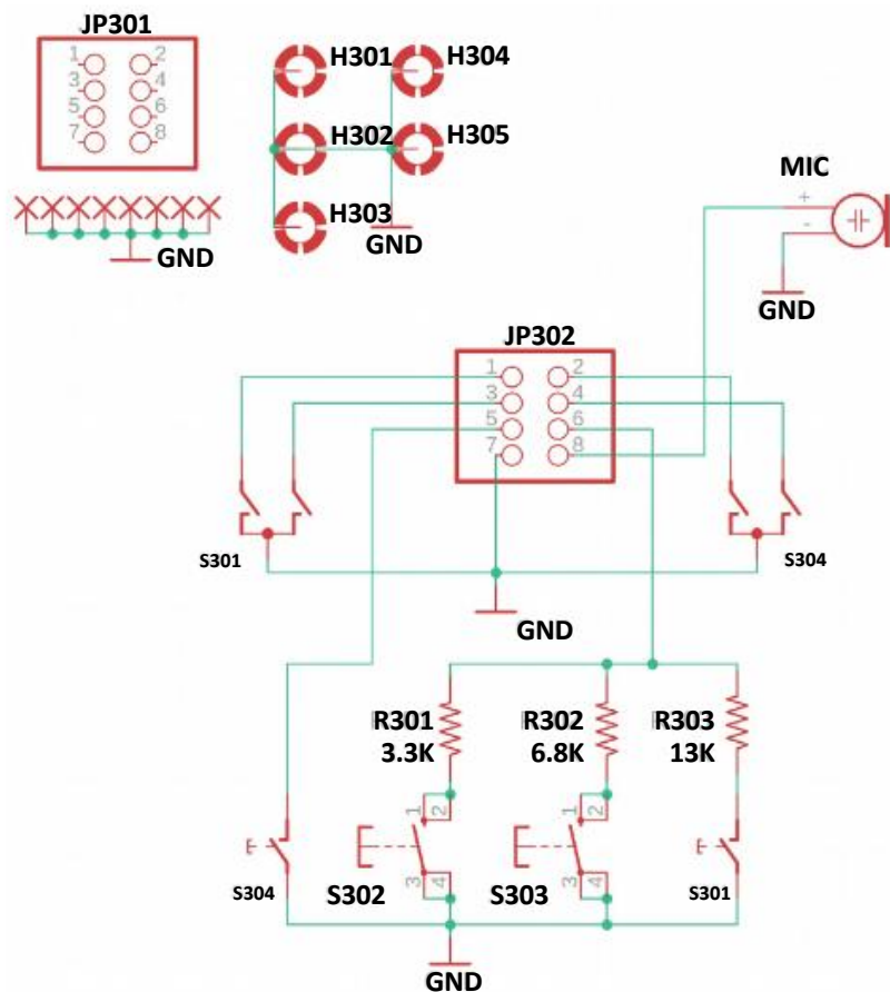
Plug-in Controls board
