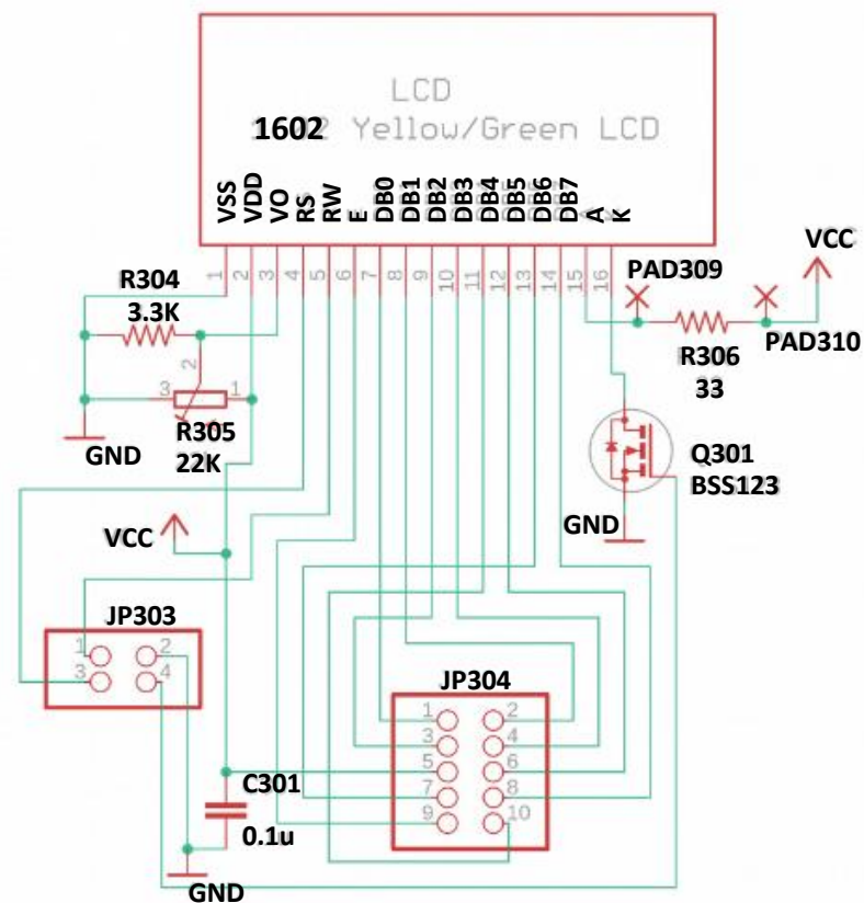
LCD board
